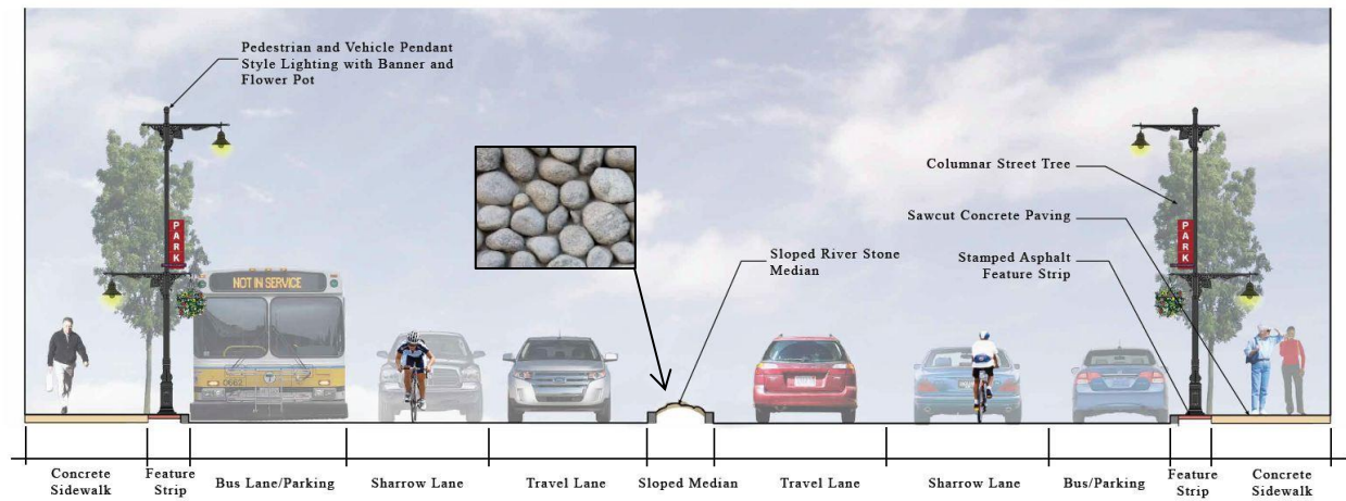
Columbia Rd Cross-Section
